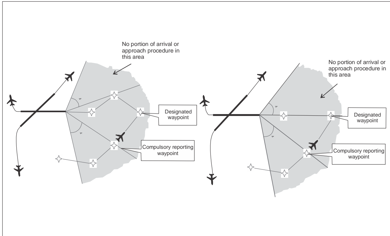
Figure 5-41. Examples of arrival protection area
